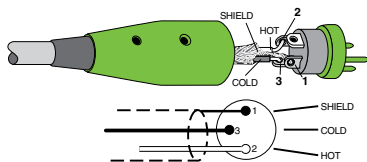
Balanced XLR Input Connector
