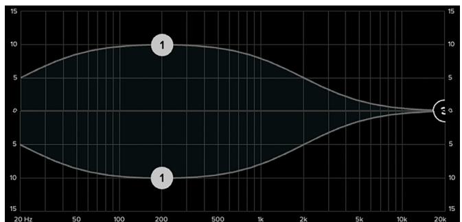
EQ OFF – Low Band (1) – 200 Hz at \pm 10 dB
